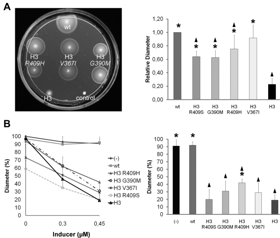
Fig. 7. Functional analysis of pseudo-revertants in semi-solid agar plates. Functional derivatives of Tsr H3 (Tsr H3* variants) isolated as described in the text were analysed in semi-solid agar plates for Tsr function and their effect on Tar function. A. UU1250 cells ( \Delta MCP) carrying the empty vector plasmid pKG116 (control), plasmid pCS12 (wild-type Tsr, wt), plasmid pTsr H3 derivative (H3) or two colonies of each of the indicated H3-derived point mutants were inoculated in tryptone semi-solid agar plates containing 12.5 \mu\text{g ml}^{-1} chloramphenicol and 0.45 \mu\text{M} sodium salicylate and then incubated for 8 h. On the left, a representative semi-solid agar plate is shown. The histogram on the right shows the ring diameter of cells bearing the H3 receptor or its pseudo-revertant relative to the ring diameter of wild-type Tsr. Significant differences ( P < 0.05 ) with respect to wild-type Tsr are indicated with \blacktriangle . Significant differences ( P < 0.05 ) with respect to the parental H3 receptor are indicated with * . The data are presented as means and standard deviations of the mean based on three images taken from independent experiments. B. UU1624 cells (lacking all MCPs except Tar) carrying the empty vector plasmid pKG116 (control), plasmid pCS12 (wild-type Tsr, wt), the Tsr H3 derivative (H3) or the indicated H3-derived point mutants were inoculated in minimal-aspartate semi-solid agar plates containing 12.5 \mu\text{g ml}^{-1} chloramphenicol and different concentrations of sodium salicylate and incubated for 20 h. The left panel shows the diameter of the resulting aspartate rings normalized to the average diameter displayed by the colonies of cells containing the empty vector with no induction. On the right, the same information is shown after induction with 0.45 \mu\text{M} sodium salicylate. Significant differences ( P < 0.05 ) with respect to the wild-type Tsr receptor are indicated with \blacktriangle . Significant differences ( P < 0.05 ) with respect to the parental H3 receptor are indicated with * . The data are presented as means and standard deviations of the mean based on three images taken from independent experiments.
