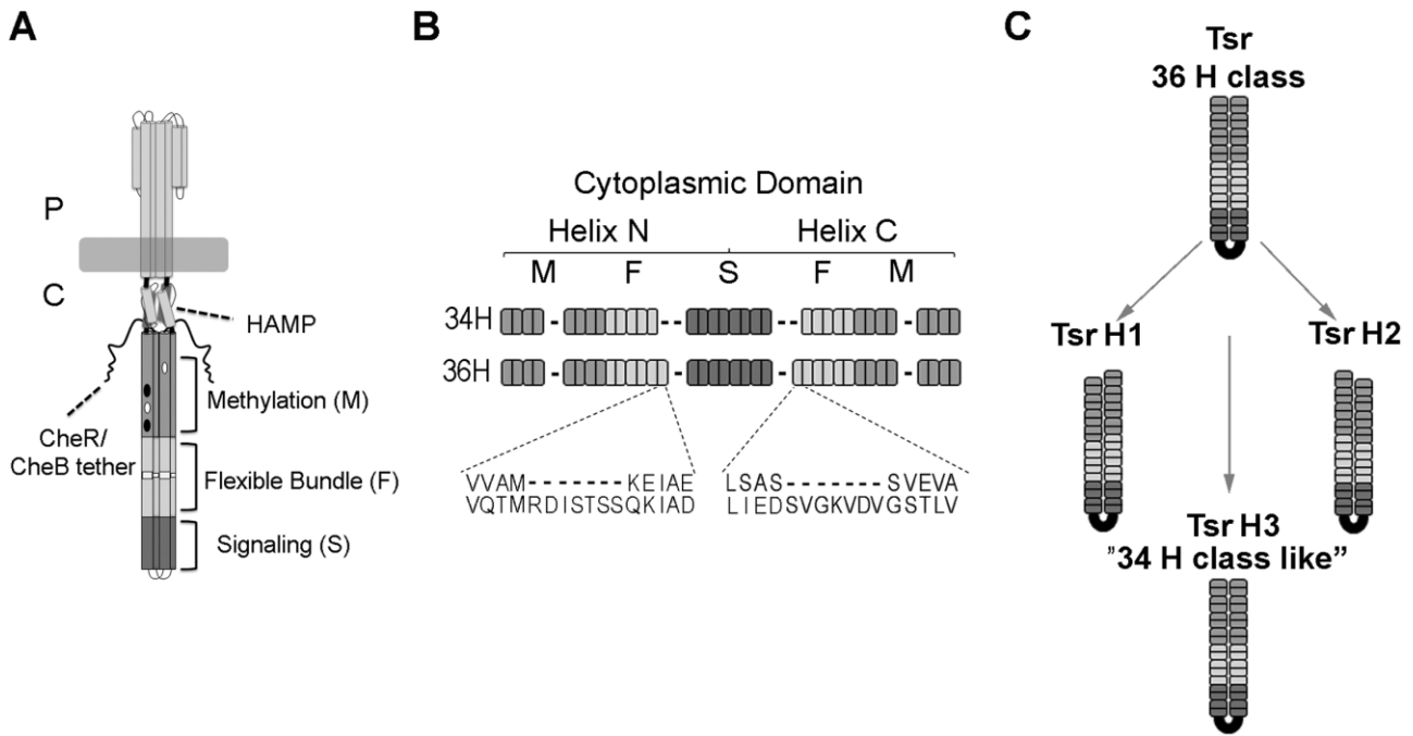
Fig. 1. Tsr-derived constructs with altered heptad content.
