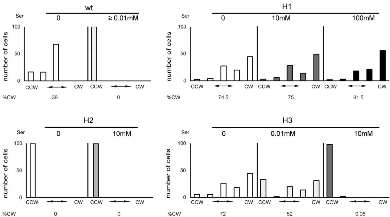
Fig. 3. Receptor-mediated control of CheA kinase. The rotational behaviour of UU1250 cells ( \Delta MCPs) expressing wild-type Tsr or its derivatives was analysed in a tethering assay. Cells were observed in the absence of stimulus or in the presence of the indicated concentrations of L-serine. One hundred cells were observed for each treatment over 15 s and classified into one of five categories, ranging from exclusively CCW to exclusively CW. The time that cells spent in CW rotation was calculated as described in Experimental procedures and is indicated below each graph. In all cases, cells were observed within less than 3 min after the addition of attractant.
