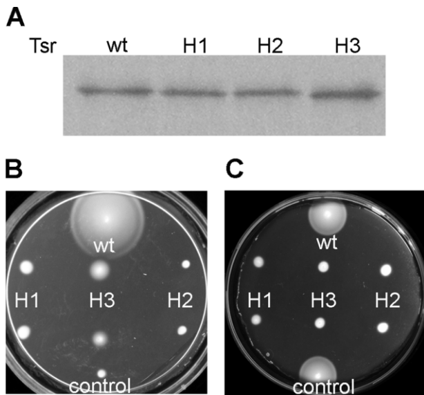
Fig. 2. Expression and functional analysis of the Tsr-variant constructs. A. Expression of Tsr-derivatives. UU1581 cells ( \Delta MCPs, \Delta che), cells carrying pCS12 (Tsr) or derivatives (H1, H2, H3) were grown to mid-log phase in the presence of 0.45 \mu M sodium salicylate. Cells were harvested by centrifugation and lysed in sample buffer. Proteins from the lysed cells was analysed by SDS-PAGE in a 12% acrylamide, 0.32% bisacrylamide gel and visualized by immunoblotting using an anti-Tsr antibody. B. Tsr function in the absence of other receptors. UU1250 cells (lacking MCPs) carrying the empty vector plasmid pKG116 (control), pCS12 (wild-type Tsr, wt) or two colonies of each Tsr derivative (H1, H2, H3) were inoculated into semi-solid T-agar plates containing 12.5 \mu g ml -1 chloramphenicol and 0.45 \mu M sodium salicylate and incubated for 8 h at 30°C. C. Tar function in the presence of Tsr derivatives. UU1624 cells (lacking all MCPs except Tar) carrying the empty vector plasmid pKG116 (control), pCS12 (wild-type Tsr, wt) or two colonies of each Tsr derivative (H1, H2, H3) were inoculated into minimal aspartate semi-solid agar plates containing 12.5 \mu g ml -1 chloramphenicol and 0.45 \mu M sodium salicylate and incubated for 20 h at 30°C.
