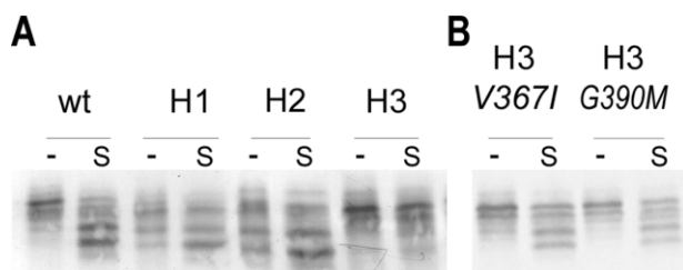
Fig. 4. Methylation response to attractant addition. A. UU1626 cells ( \Delta MCPs, \Delta cheA, \Delta cheW) carrying pCS12 (wild-type Tsr, wt), or Tsr derivatives (H1, H2, H3), were grown to mid-log phase in the presence of 0.45 \mu M sodium salicylate. Cells were harvested by centrifugation, washed twice, and resuspended in methylation buffer. After 15 min at 30°C, cells were challenged with water (-) or 100 mM L-serine (S) for 30 min. Cells were harvested and boiled in sample buffer. Proteins from the lysed cells were analysed in low bisacrylamide SDS-PAGE gels and visualized by immunoblotting using an anti-Tsr antiserum. Faster-migrating bands represent more-highly methylated species. B. The same experiment was carried out with UU1626 cells expressing the pseudo-revertants Tsr H3 V367I or Tsr H3 G390M.
