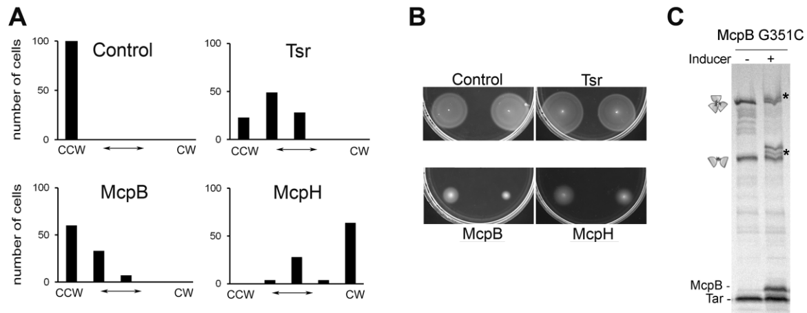
Fig. 8. Expression of McpB or McpH from Rhodospirillum rubrum 2.4.1 in E. coli .
